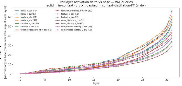
Figure 3: Same as Figure 2, on held-out validation queries. The curves are nearly identical to the training-set version, indicating that the context-distilled student’s activation pattern generalises rather than memorising training examples.
