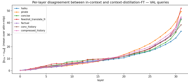
Figure 5: Same as Figure 4, on held-out validation queries. Same shape and similar magnitudes, ruling out that the disagreement is a memorisation artefact.
