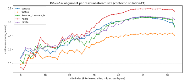
Figure 1: RMSNorm cosine between v^{\text{ctx}} and v^{\text{dist}} at each of the 64 residual-stream sites in Llama-3.1-8B (32 layers, post-attention followed by post-MLP per layer; site 2\ell = post-attn at layer \ell , site 2\ell + 1 = post-MLP at layer \ell ). Averaged over a held-out probe set of 28 queries per context. One line per context type.
