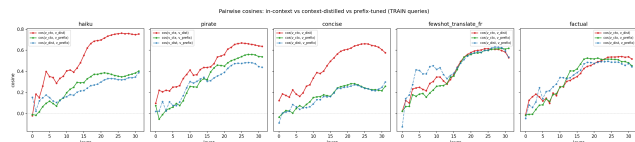
Figure 8: Pairwise cosine similarities between v^{\text{ctx}} (in-context) and the perturbations from full distillation v^{\text{dist}} and prefix tuning v^{\text{prefix}} . Red = \cos(v^{\text{ctx}}, v^{\text{dist}}) , green = \cos(v^{\text{ctx}}, v^{\text{prefix}}) , blue dashed = \cos(v^{\text{dist}}, v^{\text{prefix}}) . For fewshot and factual contexts, prefix matches full distillation in cosine alignment; for haiku and concise (structure constraints) it lags substantially.
