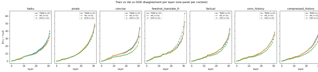
Figure 6: Per-layer \|v^{\text{ctx}} - v^{\text{dist}}\| on TRAIN (solid), VAL (dashed), and OOD MMLU-Pro (dotted) queries, one panel per context. Across every context the three curves nearly overlap: the student perturbs the residual stream by essentially the same amount on academic multiple-choice questions as on the queries it was trained on. The same in-context vs context-distilled disagreement pattern shows up regardless of input distribution.
