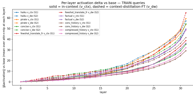
Figure 2: Per-layer activation change vs base, on train queries. Solid = \|v^{\text{ctx}}\| (in-context). Dashed = \|v^{\text{dist}}\| (context-distilled). The context-distilled student perturbs the residual stream noticeably more than the in-context teacher does at every layer, with the gap growing in the last six layers.
