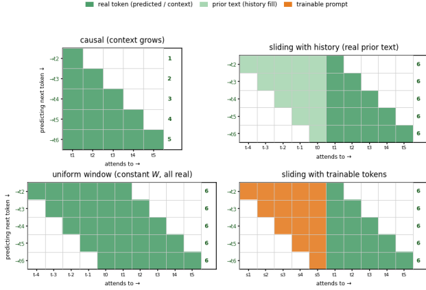
Figure 2: Four continued-pretraining regimes, each a window of attention (rows = the token being predicted; the right number is its working-memory size). Top: the standard causal mask, where context grows with position; and a sliding window of constant width W whose cold start is filled with real prior text (light green). Bottom, our constant-memory variants: a uniform window , where every token is conditioned on exactly W real tokens via fixed-length training (predicting only each window’s last token, so it also runs on a recurrence); and a sliding window with trainable tokens , where a trainable startup prompt (orange) fills the cold start in place of real history and slides out as content accumulates. Older real context must be carried by the weights.
