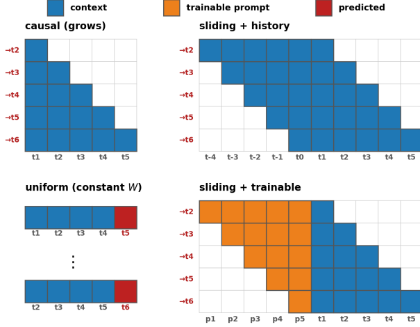
Figure 2: Four continued-pretraining regimes (token labels coloured grey for context and crimson for predicted ). Top , attention masks (rows = a predicting step, columns = attended positions; both predict every token): the standard causal mask, where context grows with position; and a sliding window of constant width W whose cold start is filled with real prior text (blue, the same as content — history is just earlier context). Bottom : the uniform window is not an attention mask but fixed-length training — a stack of fixed-length sequences (two successive ones shown, right-aligned, \vdots for the rest), each predicting only its last token (crimson) from its preceding context, so it also runs on a recurrence; and a sliding window with trainable tokens , whose cold start is filled by a trainable startup prompt (orange) that slides out as content accumulates. Older real context must be carried by the weights.
