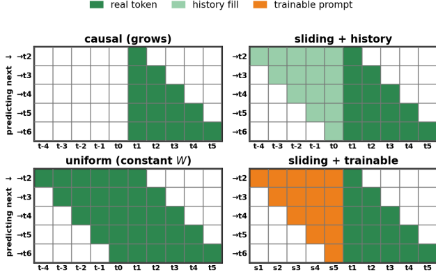
Figure 2: Four continued-pretraining regimes, each a window of attention (rows = the token being predicted, columns = the positions it attends; a short prefix region plus the content tokens). All three windowed variants hold a constant width W ; causal grows. Top : the standard causal mask, where context grows with position; and a sliding window of constant width W whose cold start is filled with real prior text (light green). Bottom, our constant-memory variants : a uniform window , where every token is conditioned on exactly W real tokens via fixed-length training (predicting only each window’s last token, so it also runs on a recurrence); and a sliding window with trainable tokens , where a trainable startup prompt (orange) fills the cold start in place of real history and slides out as content accumulates. Older real context must be carried by the weights.
