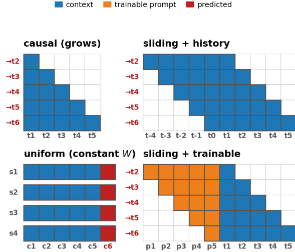
Figure 2: Four continued-pretraining regimes (token labels coloured grey for context and crimson for predicted ). Top, attention masks (rows = a predicting step, columns = attended positions; both predict every token): the standard causal mask, where context grows with position; and a sliding window of constant width W whose cold start is filled with real prior text (blue, the same as content — history is just earlier context). Bottom: the uniform window is not an attention mask but fixed-length training — four separate windows, each conditioning on exactly W real tokens and predicting only its last token (crimson, c_6 ), so it also runs on a recurrence; and a sliding window with trainable tokens , whose cold start is filled by a trainable startup prompt (orange) that slides out as content accumulates. Older real context must be carried by the weights.
