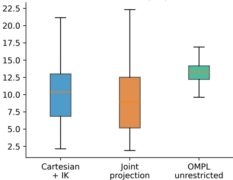
Joint travel: sum |\Delta q| (rad)
