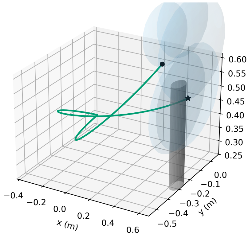
OMPL unrestricted
