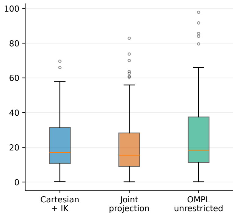
Minimum robot-world clearance (mm)
