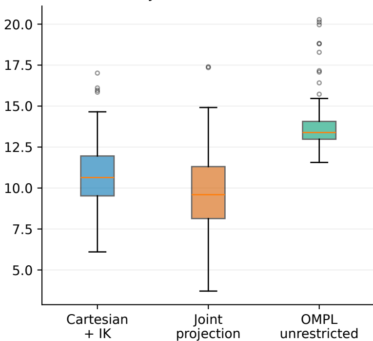
Joint travel (rad)
