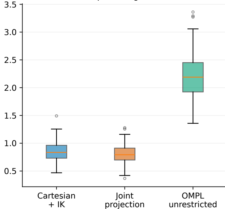
EE path length (m)
