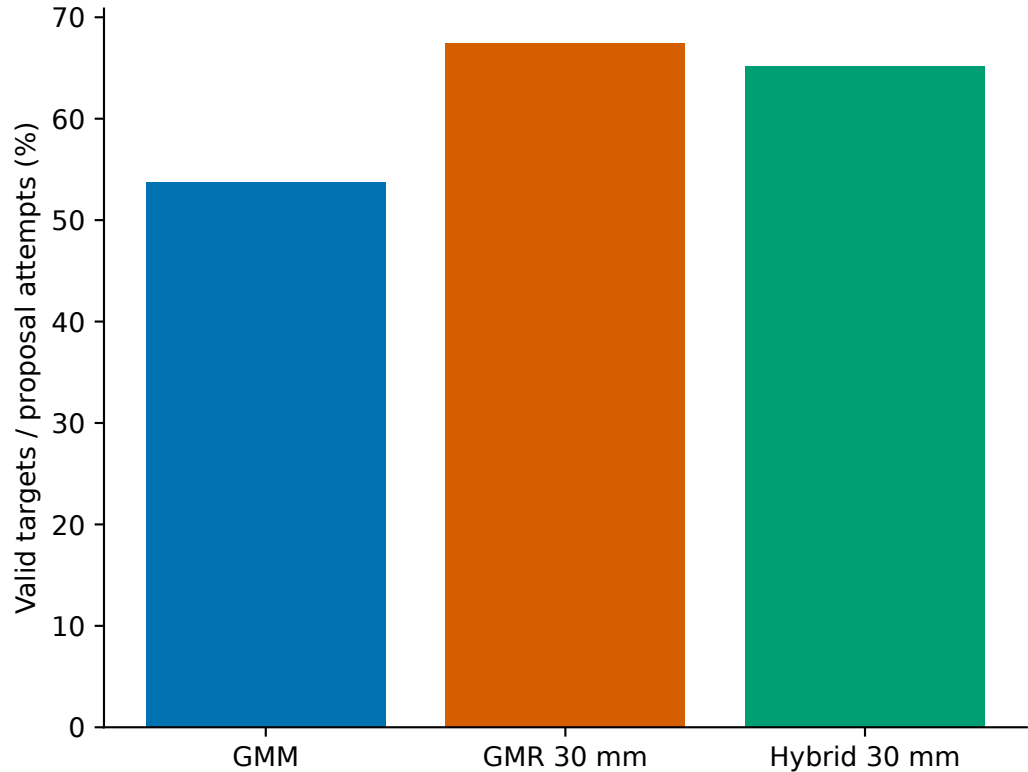
Sampling efficiency
