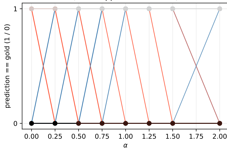
B) Per-user correctness vs \alpha (blue: flipped; red: broken)
