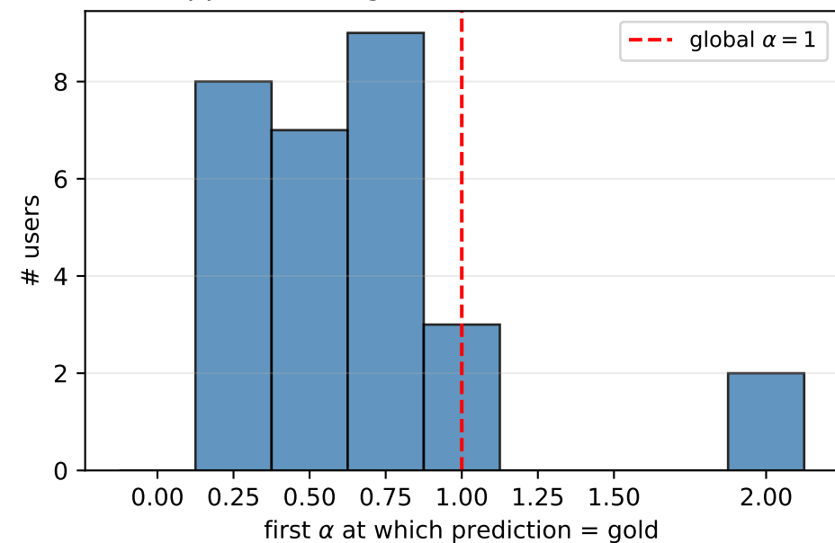
C) Phase-boundary distribution (29 flipped users, global \alpha = 1 misses all of them)
