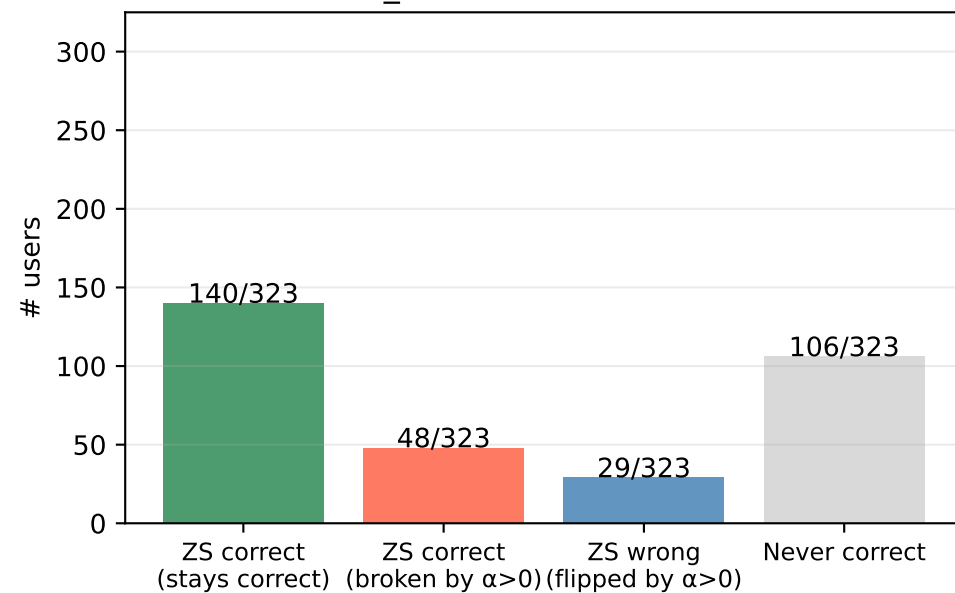
A) Per-user effect of steering net \Delta_{\text{users}} = +29 - 48 = -19
