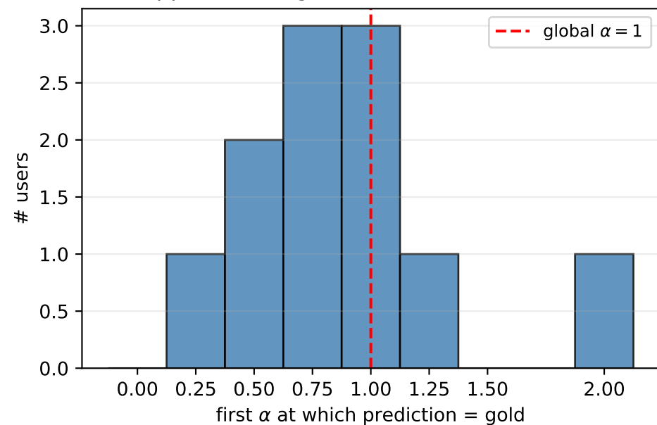
C) Phase-boundary distribution (11 flipped users, global \alpha = 1 misses all of them)
