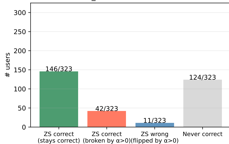
A) Per-user effect of steering net \Delta_{\text{users}} = +11 - 42 = -31
