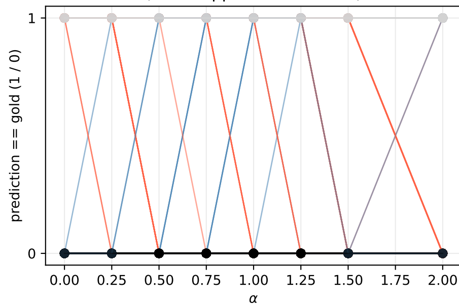
B) Per-user correctness vs \alpha (blue: flipped; red: broken)
