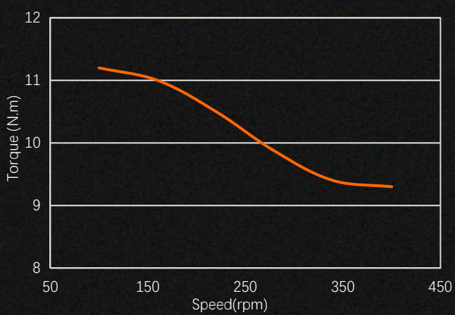
热平衡态T-N曲线 Thermal equilibrium state T-N curve (200mmX200mm铝散热板)
