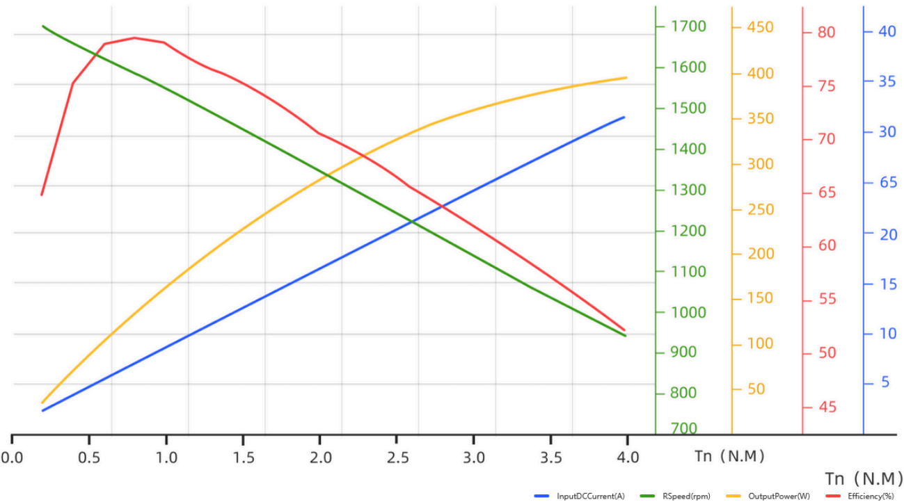
FOC Control Characteristics Graph
