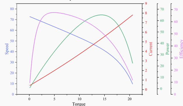
Motor performance curve
