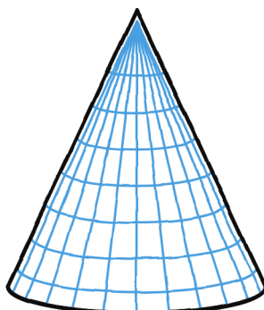
CONE RINGS SHRINK TO THE TIP
