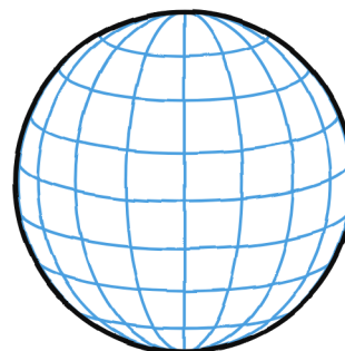
SPHERE CURVES BOTH WAYS
