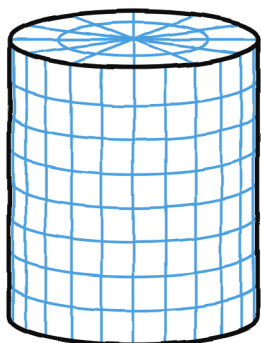
CYLINDER RINGS AROUND, LINES DOWN
