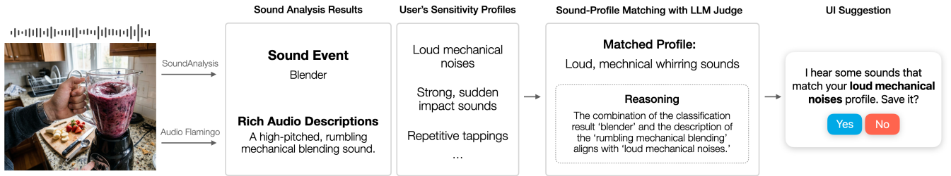
Figure 5: Sona’s trigger discovery pipeline. When an unsupported sound is detected, the system generates a description and matches it against user-defined sensitivity profiles to determine whether it should be saved for later personalization.
