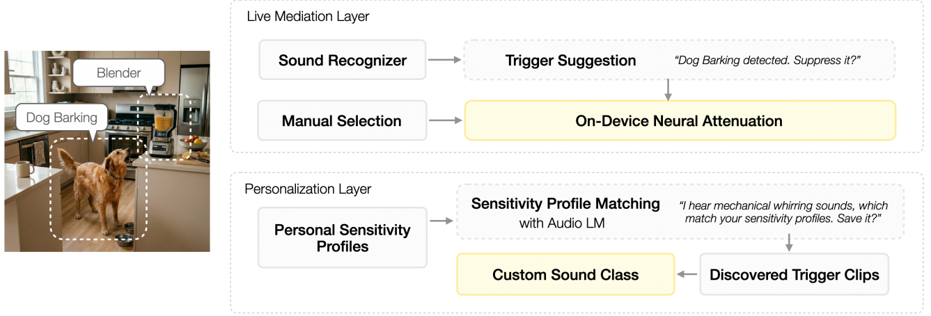
Figure 4: Sona’s two-layer system architecture. The Live Mediation Layer runs on-device: users select target sounds manually or accept suggestions from a sound recognizer, and the neural attenuation model reduces the selected sounds at an adjustable strength while preserving the rest of the scene. The Personalization Layer extends the built-in sound set: users describe personal triggers as sensitivity profiles, Sona matches audio-language-model descriptions of the live soundscape against these profiles and prompts users to save matching clips, and users create custom sound classes from saved or manually recorded examples.
