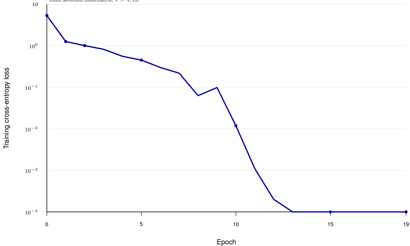
Loss-selected StateCache, k = 4 , L6
