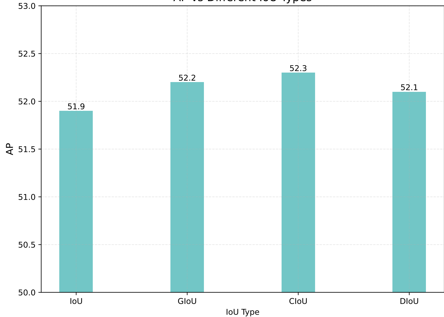
AP vs Different IoU Types
