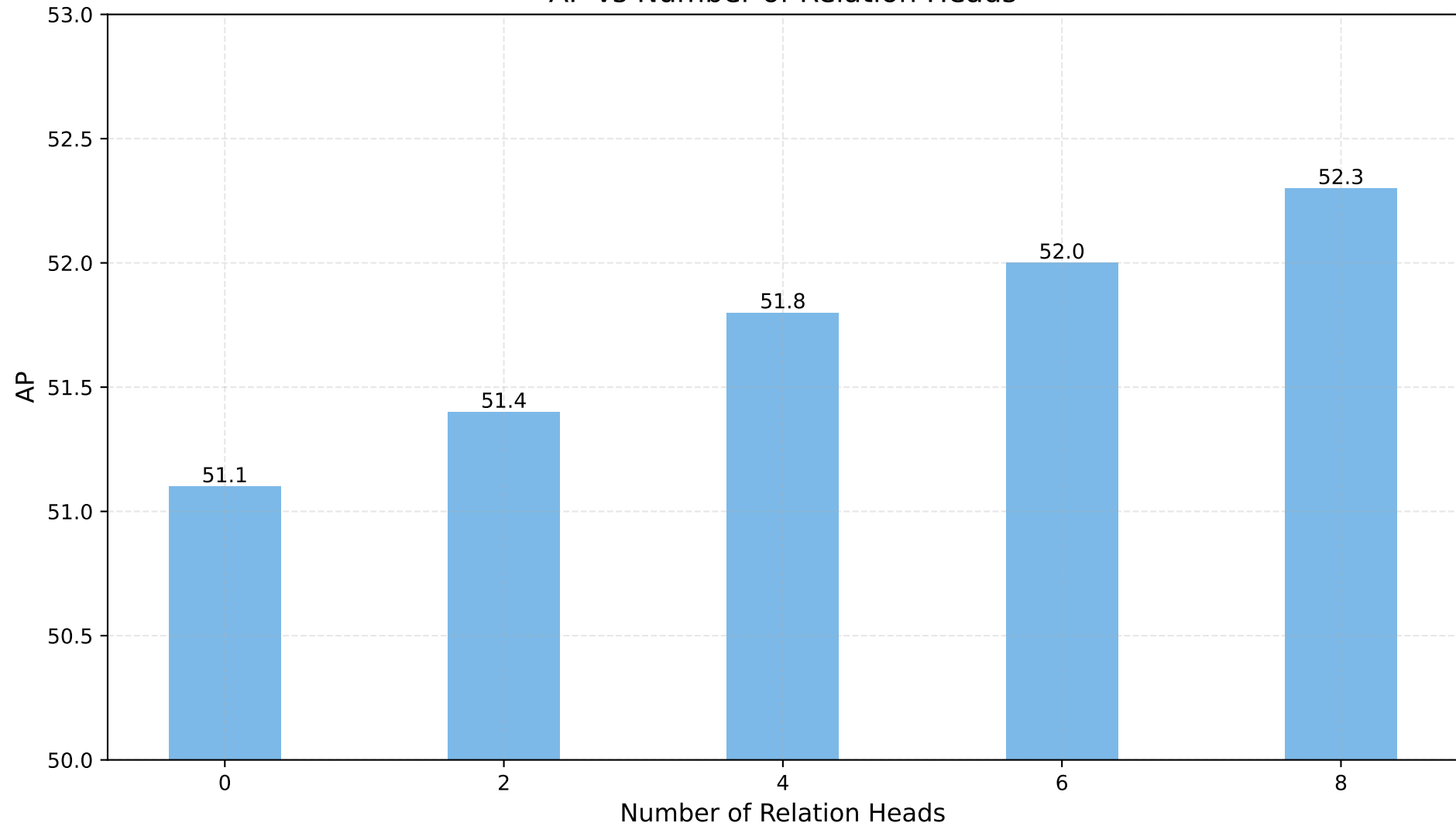
AP vs Number of Relation Heads
