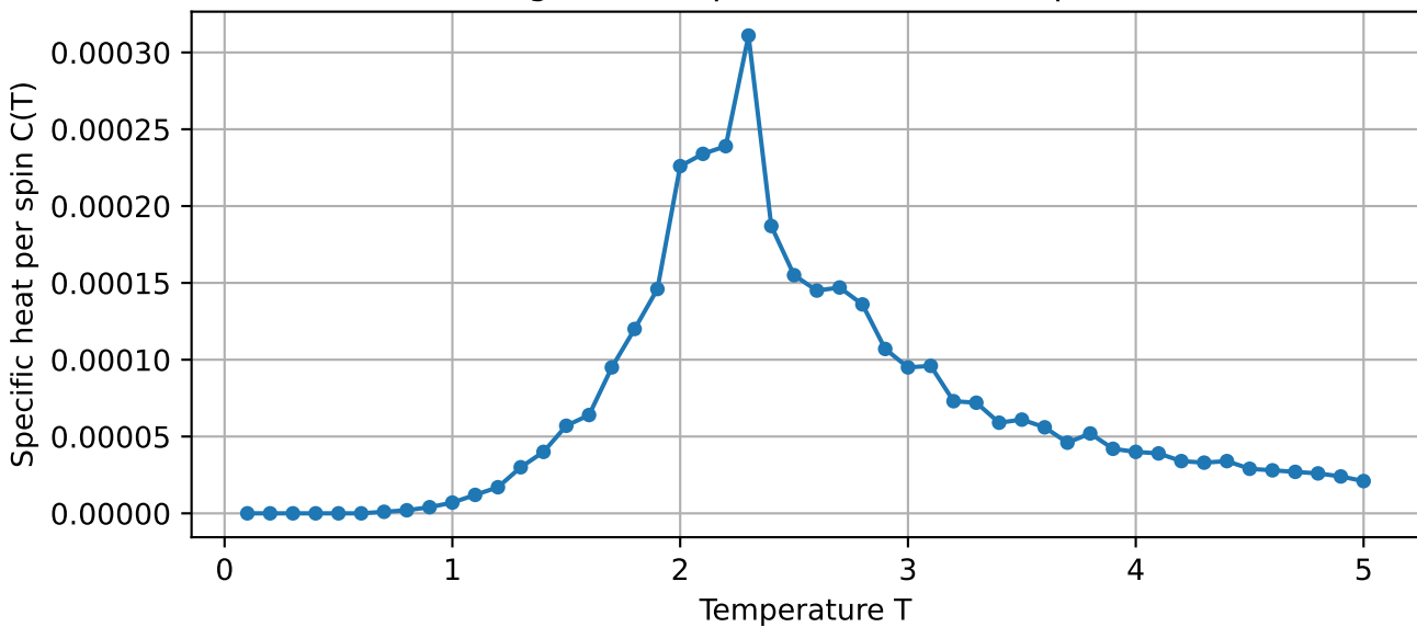
2D Ising Model: Specific Heat vs Temperature
