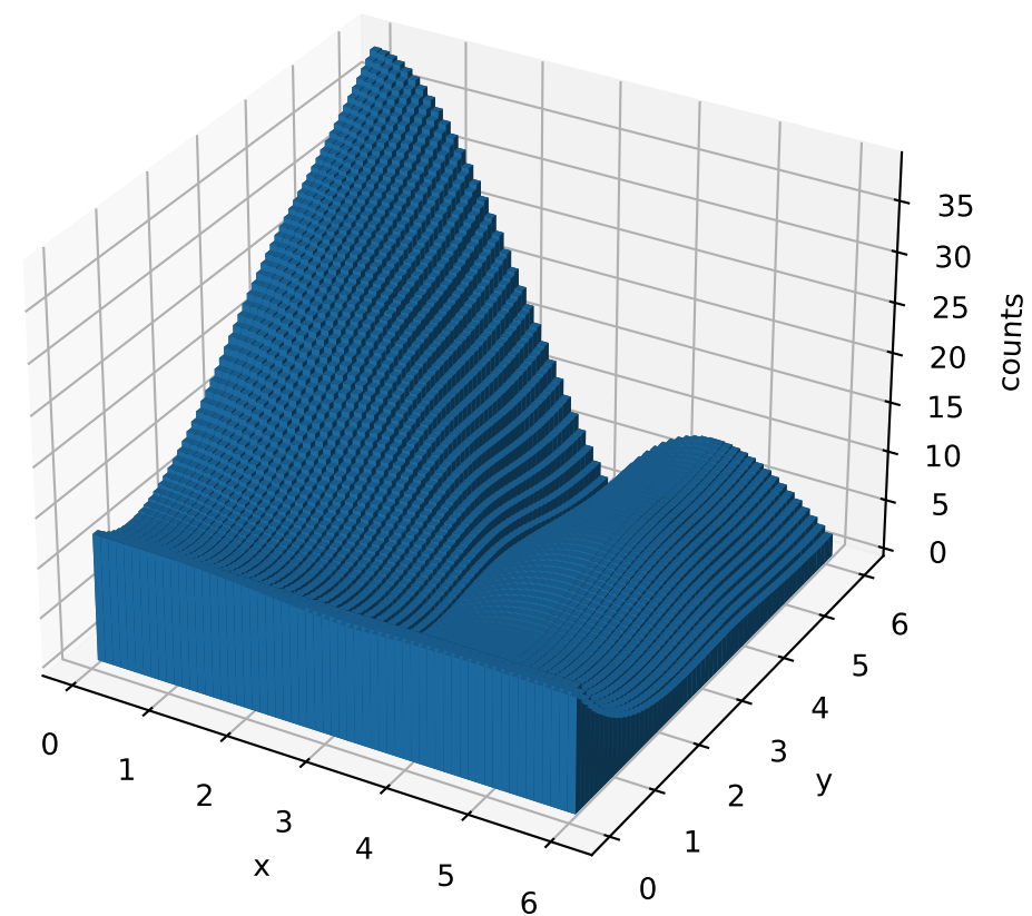
Data - Best-fit Background
