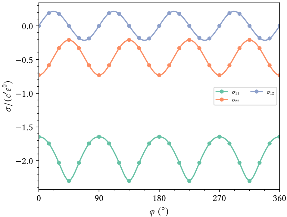
\varepsilon_{11}, A_Z = 8 : interior stress vs. matrix rotation
