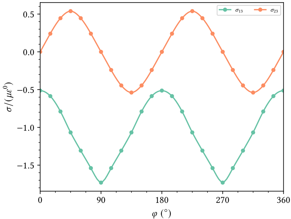
\varepsilon_{13}, c_{44}/c_{55} = 8 : interior stress vs. matrix rotation
