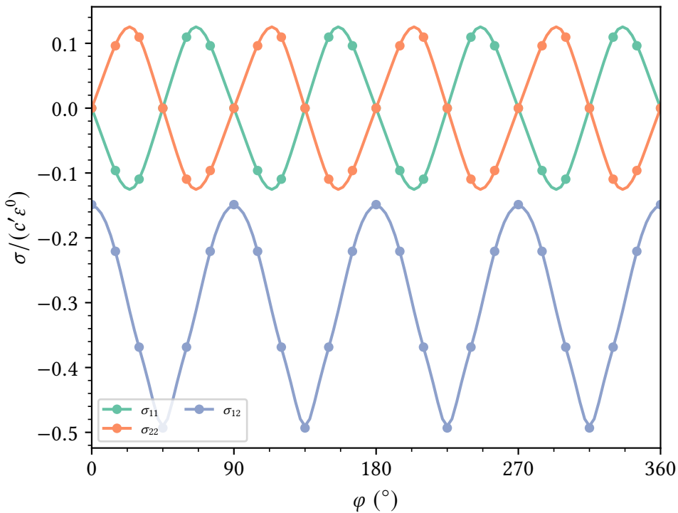
\varepsilon_{12}, A_Z = 0.125 : interior stress vs. matrix rotation
