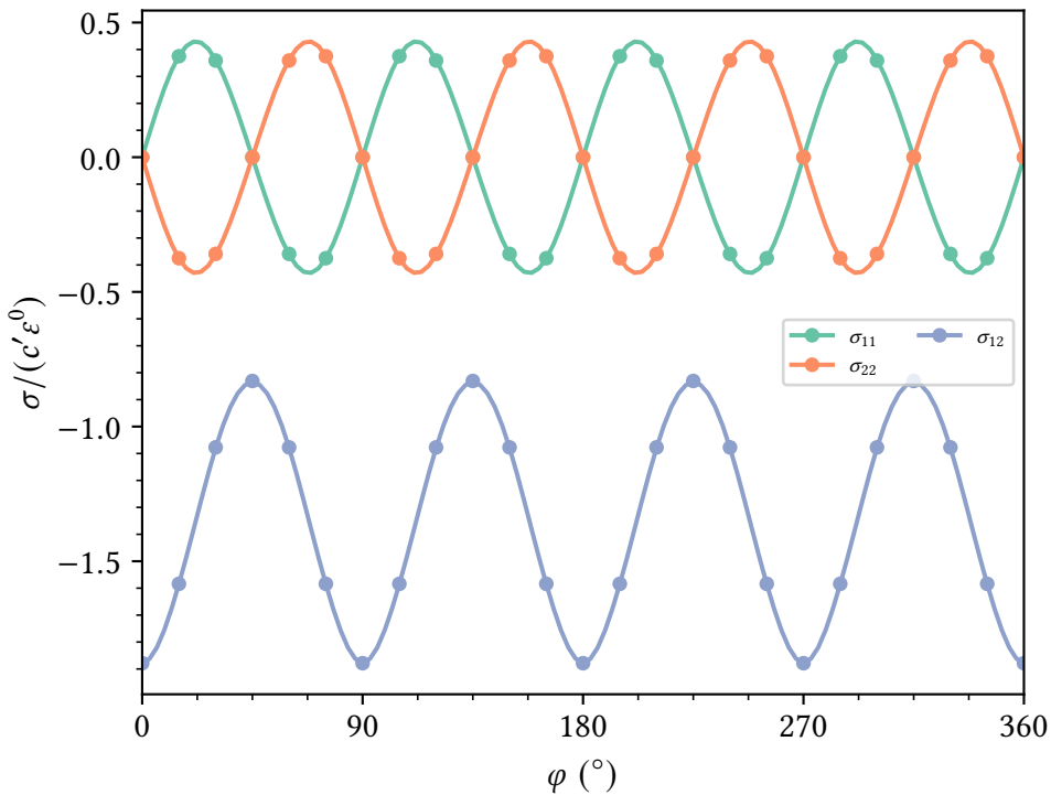
\varepsilon_{12}, A_Z = 8 : interior stress vs. matrix rotation
