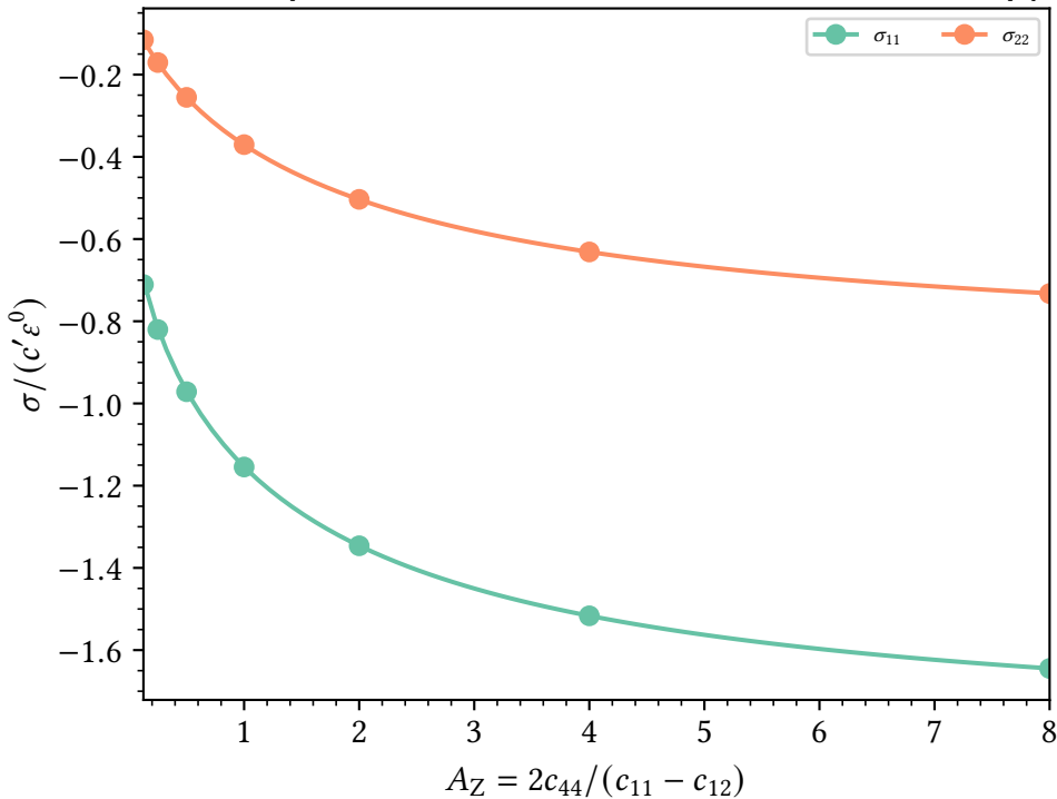
anisotropic matrix, \varepsilon_{11} : interior stress vs. anisotropy
