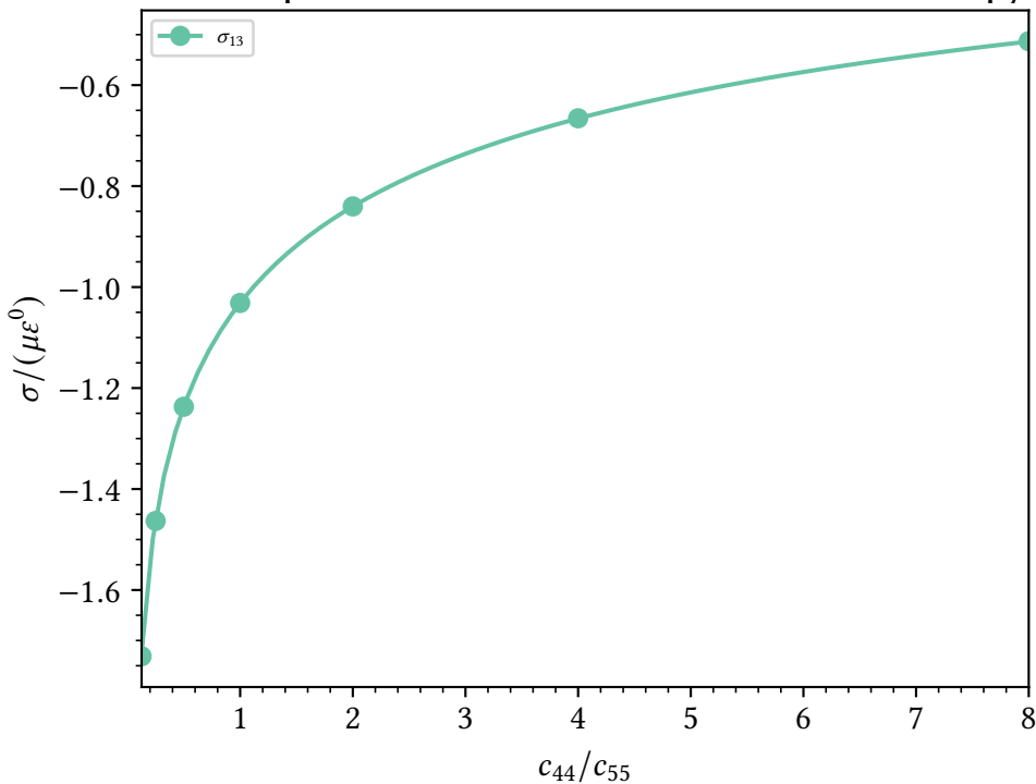
anisotropic matrix, \varepsilon_{13} : interior stress vs. anisotropy
