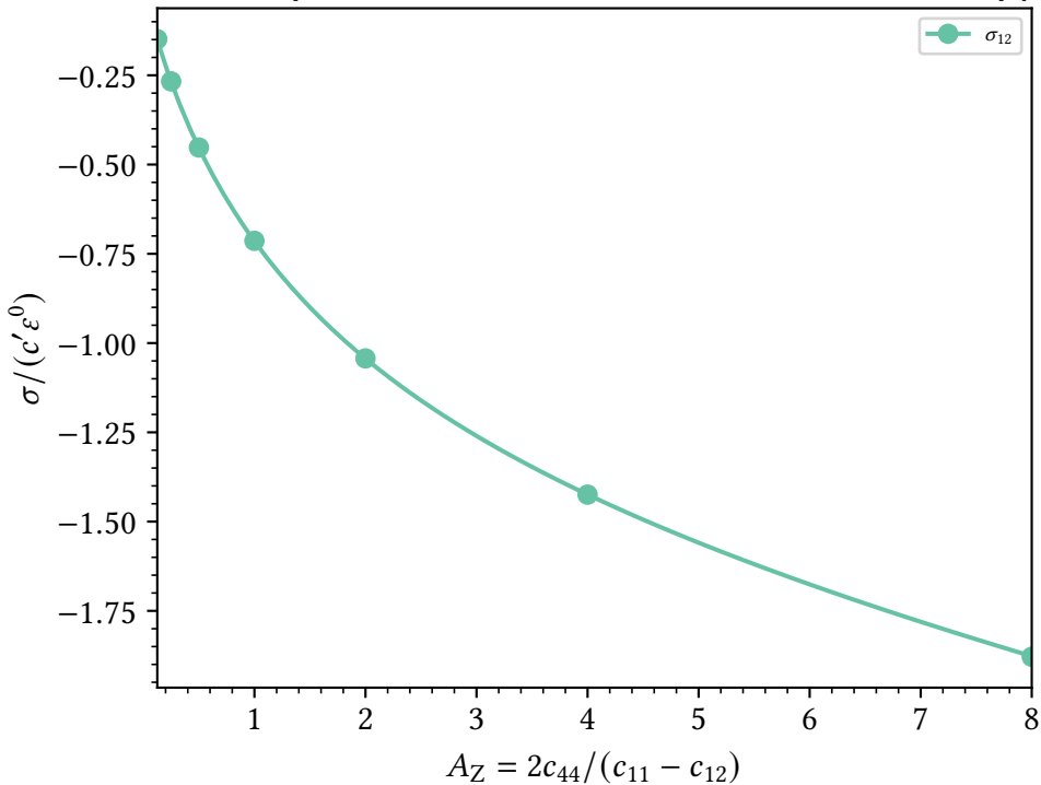
anisotropic matrix, \varepsilon_{12} : interior stress vs. anisotropy
