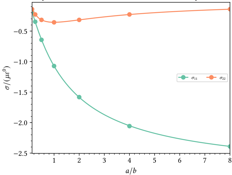
elliptical inclusion, \varepsilon_{11} : interior stress vs. aspect ratio
