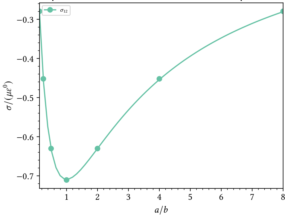
elliptical inclusion, \varepsilon_{12} : interior stress vs. aspect ratio
