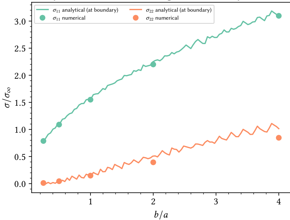
elliptical hole, moment: edge stress vs. aspect ratio
