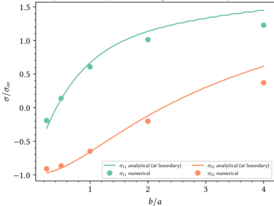
elliptical hole, pressure: edge stress vs. aspect ratio
