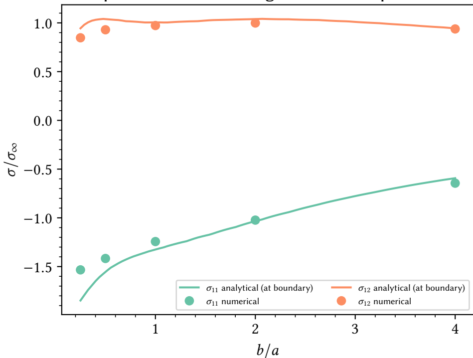
elliptical hole, shear: edge stress vs. aspect ratio
