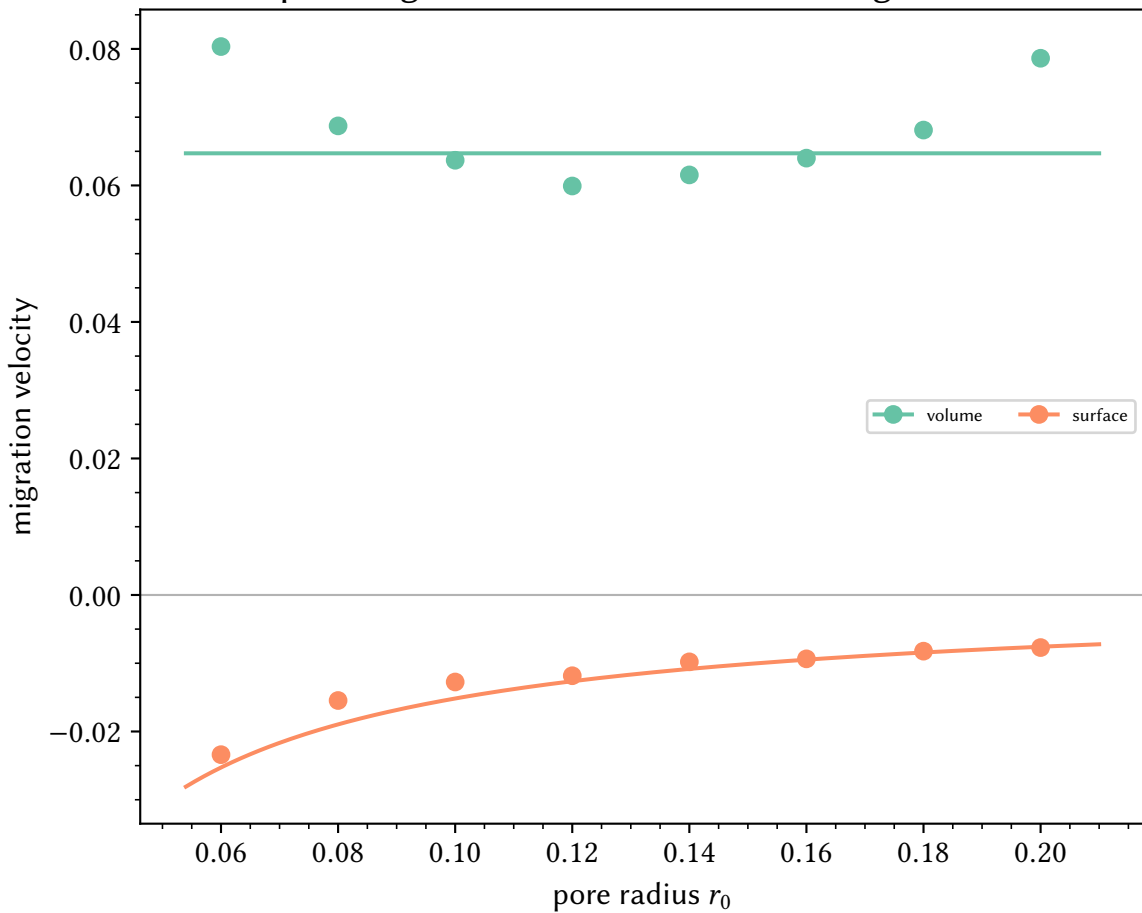
pore migration under a remote stress gradient
