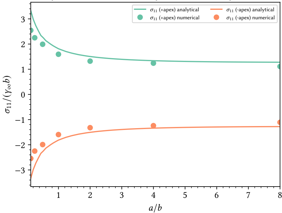
elliptical hole, moment: apex stress vs. aspect ratio
