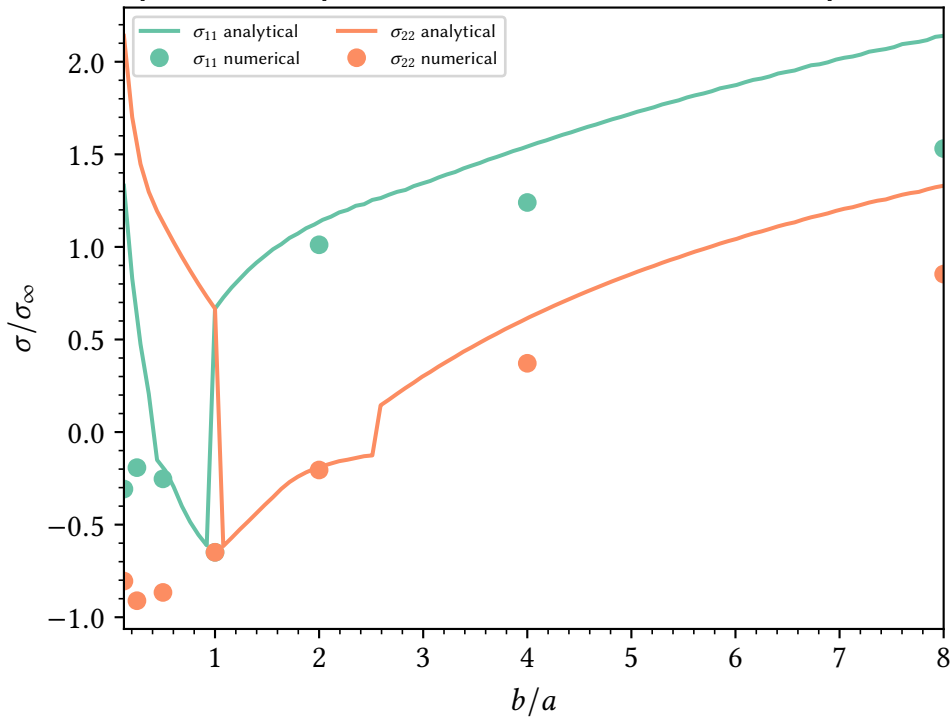
elliptical hole, pressure: maximum stress vs. aspect ratio
