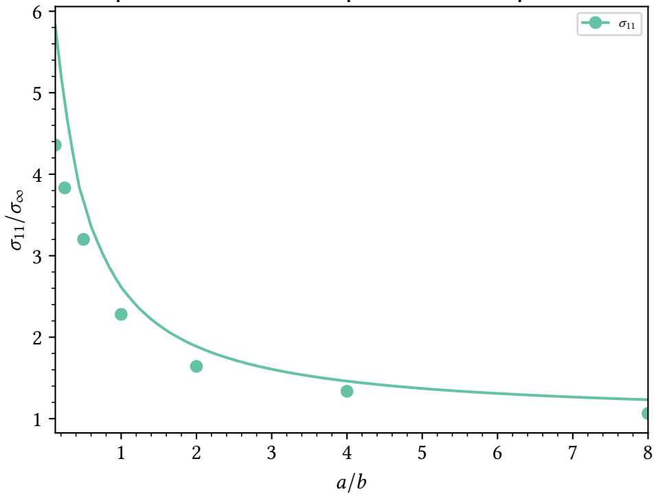
elliptical hole, tension: apex stress vs. aspect ratio
