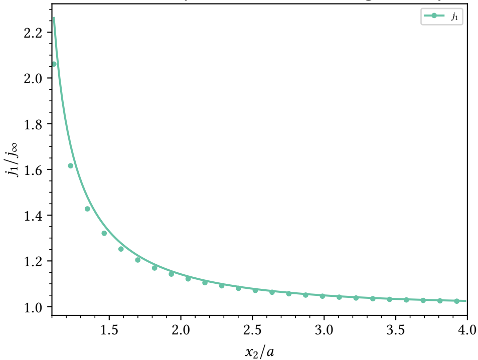
current density ahead of an insulating crack tip
