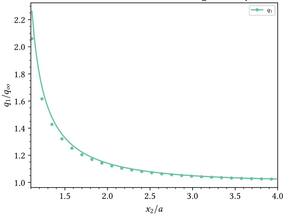
heat flux ahead of an insulating crack tip
