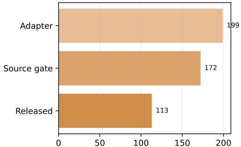
AppWorld
