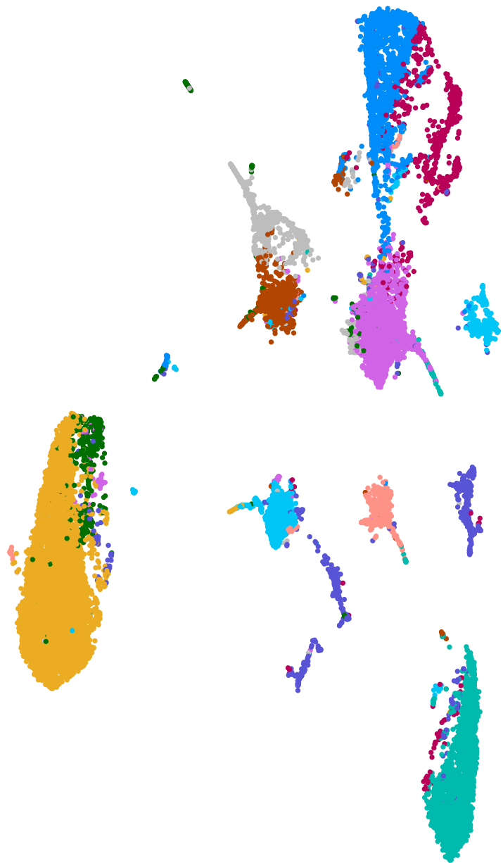
UMAP of male NSD samples
