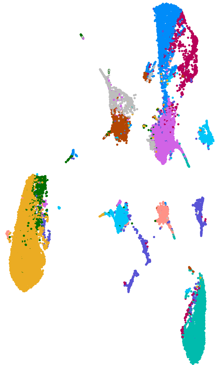
UMAP of all male samples
