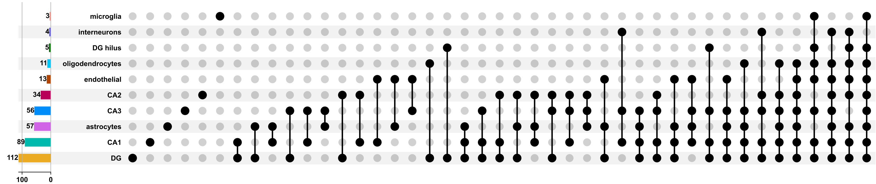
Number of DEGs
