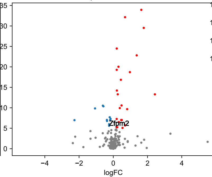
CA3, p-value=2.41E-06
