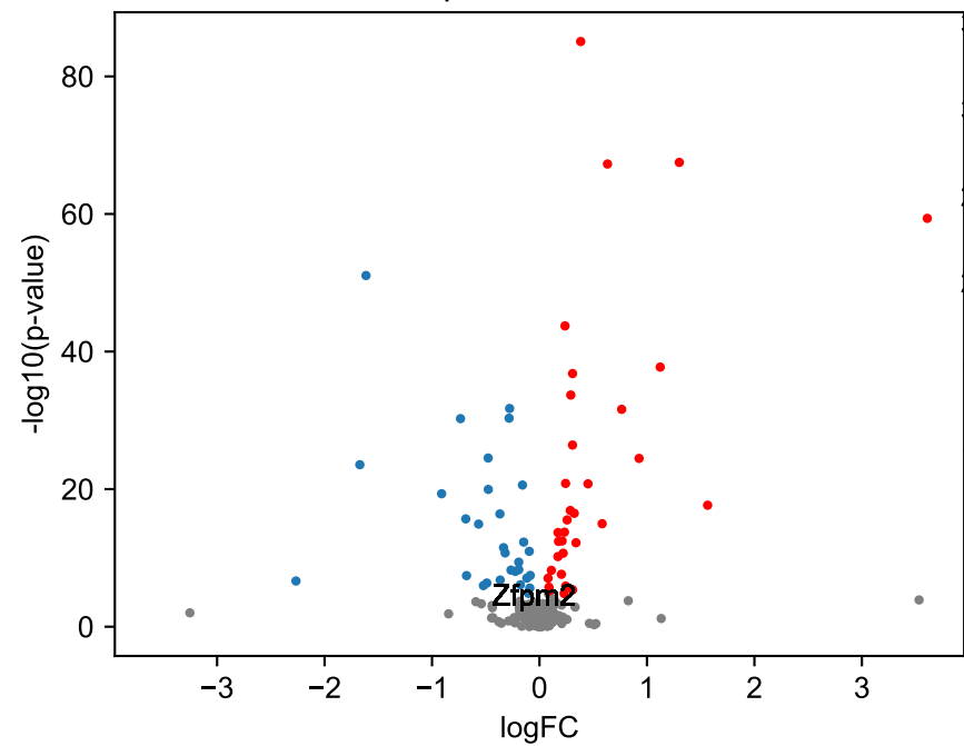
CA1, p-value=8.30E-04
