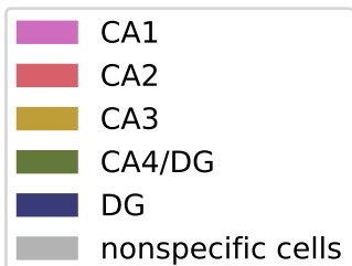
Clustering, k=15
