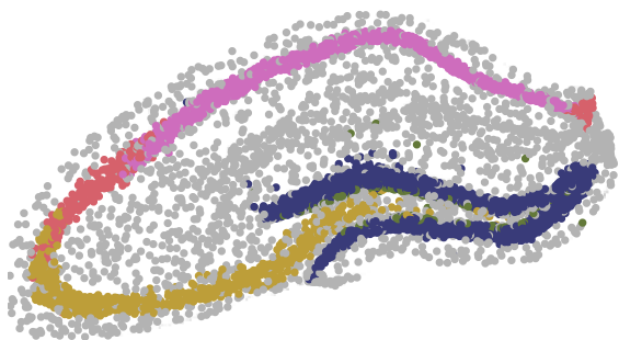
Clustering, k=15
