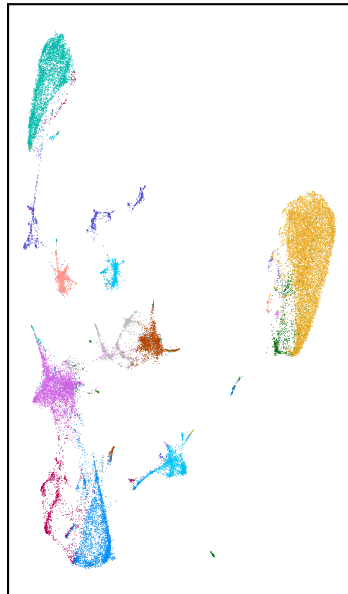
UMAP of all male samples
