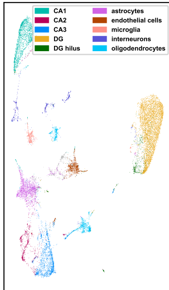
UMAP of male SD samples
