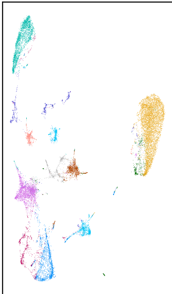
UMAP of male NSD samples
