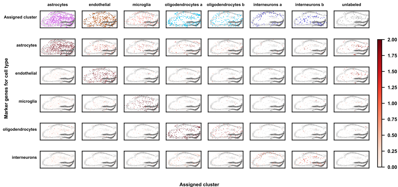
Mean z-score for cell type marker genes, SD-YW-1_ROI_A2_hippocampus
