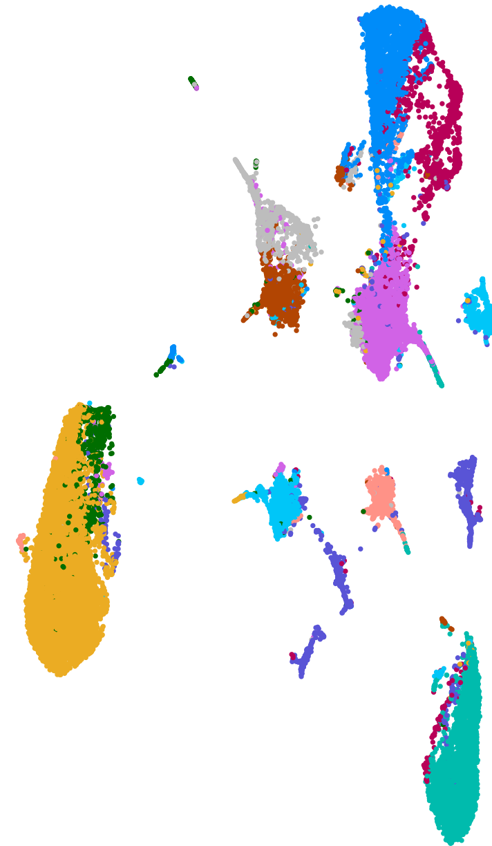
UMAP of all male samples
