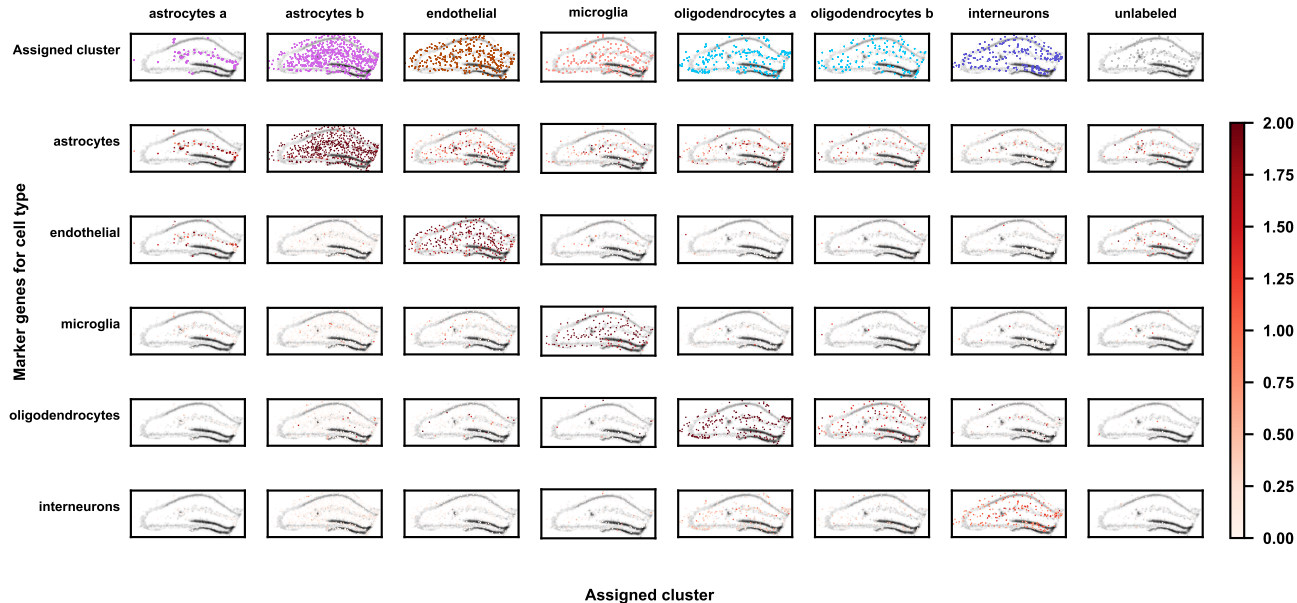
Mean z-score for cell type marker genes, SD-2
