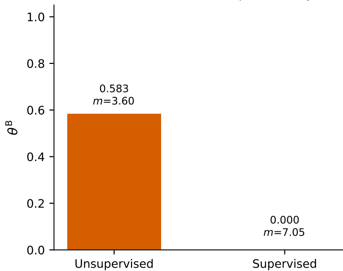
Selected-bad first-hit probability
