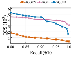
Figure 14: QPS-Recall@k across result sizes.
